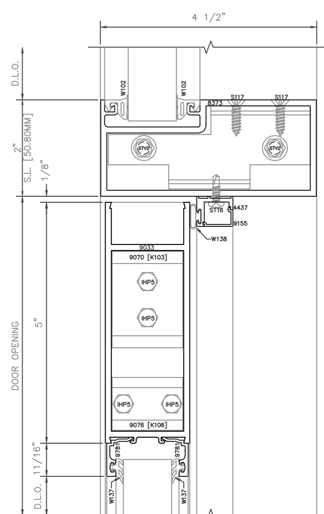
1 DOOR HEAD DETAIL SCALE: 6" = 1'-0"
