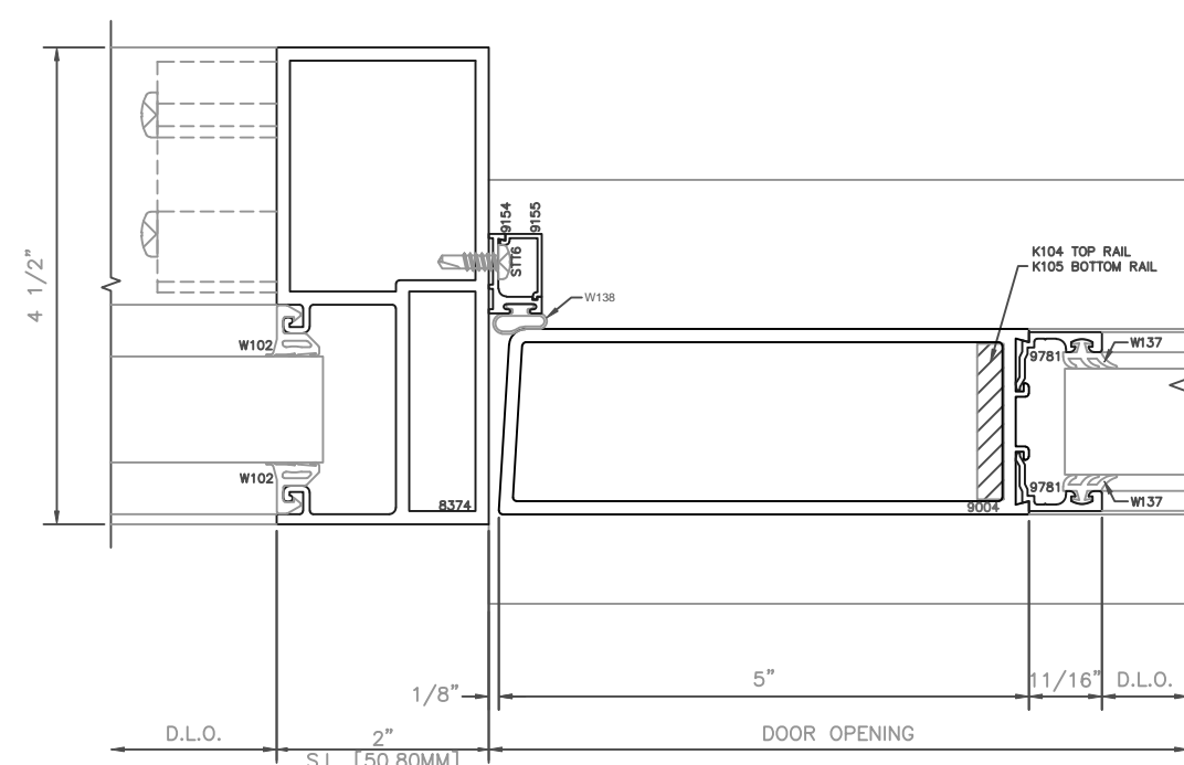
3 DOOR JAMB DETAIL SCALE: 6" = 1'-0"
